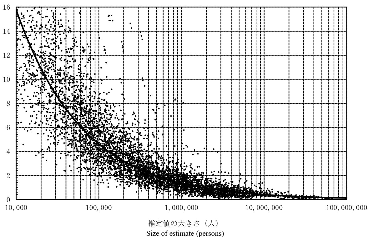
Distribution of standard error ratios by size of estimate for Japan
